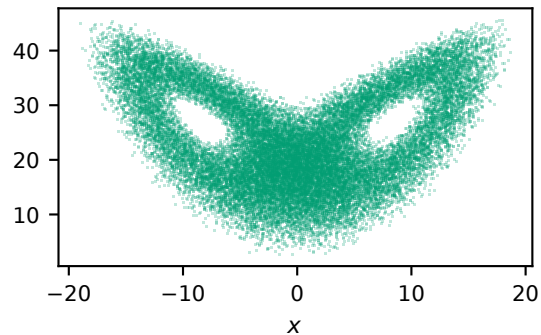
speedx2: attractor (x, z) — identical
