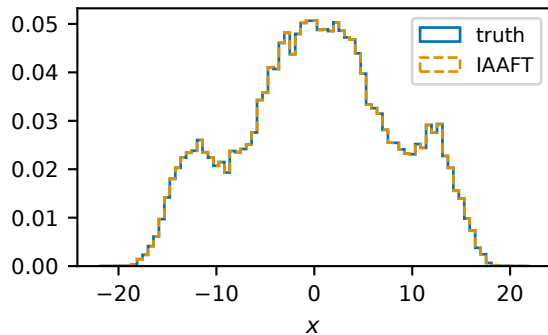
marginal of x — exactly equal
