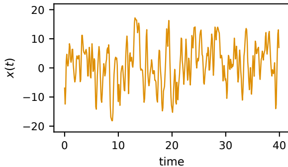
marginal of x — exactly equal
