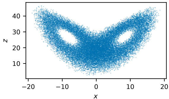
truth: attractor (x, z)
