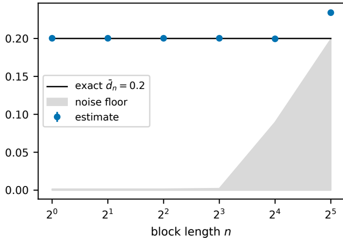
iid Bern(0.3) vs. iid Bern(0.5)
