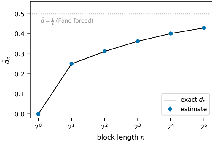
iid( \frac{1}{2} ) vs. period-2 alternation
