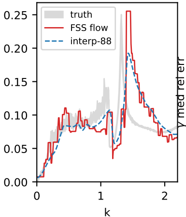
Nik target: both inaccurate
