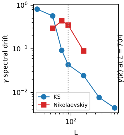
drift: fast KS, slow Nik
