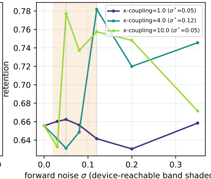
(b) coupling tunes the optimum to the chip's noise level
