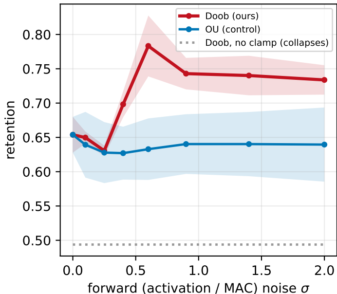
(a) mechanism survives forward noise (the hardware-relevant case)
