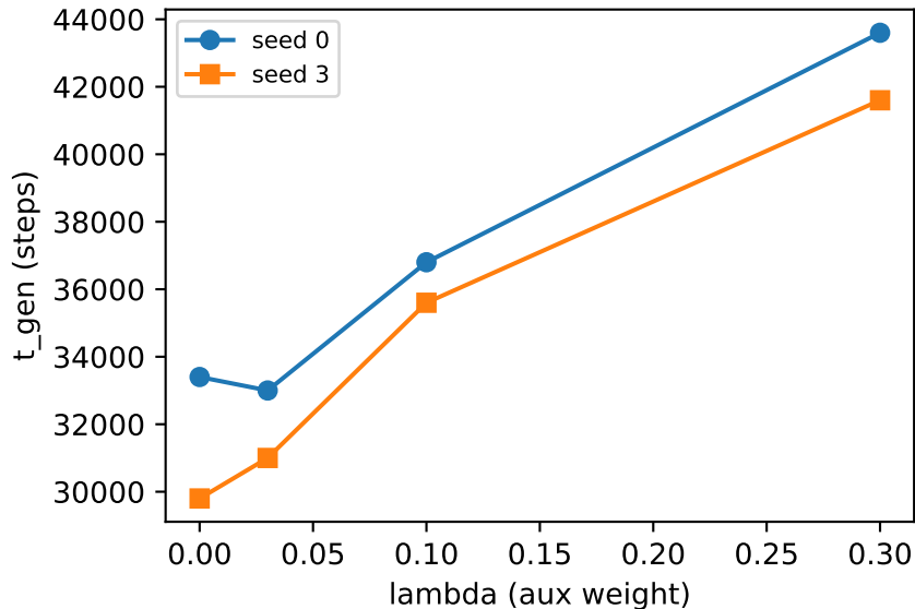
Free-norm dose: no dose wins
