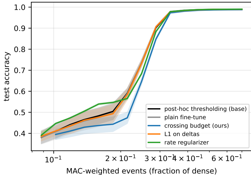
row-sequential MNIST
