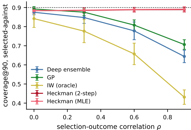
(b) coverage vs \rho (instrument present)
