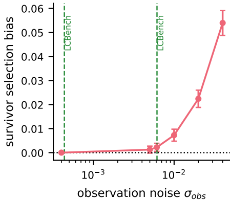
(b) bias vs noise (rung 1, \eta = 3 )
