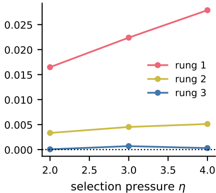
(c) bias vs \eta ( \sigma = 0.02 )
