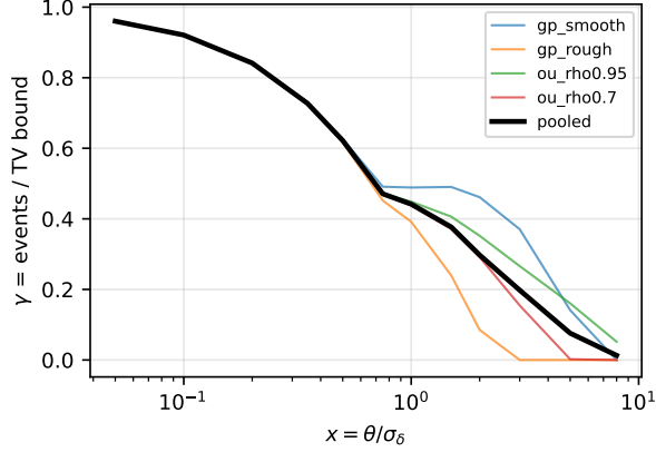
Figure 2: Send-on-delta correction. Measured event rate over the TV/ \theta bound, \gamma , vs x = \theta/\sigma_\delta for four synthetic process families (3 seeds each). For x \leq 0.5 the curves collapse (spread 0.5%); beyond x \approx 1 the tail of the increment distribution takes over and process-dependence sets in.
