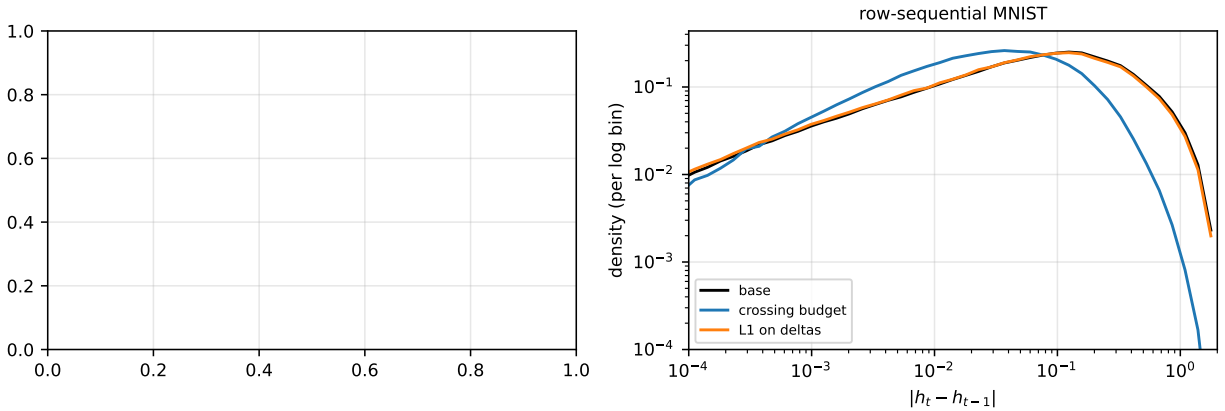
Figure 7: Mechanism check: increment histograms. The budget compresses the entire |\Delta h| distribution (scale shrink); L1-delta mildly sharpens it. Neither restructures the dynamics in a way that survives threshold re-scaling.
