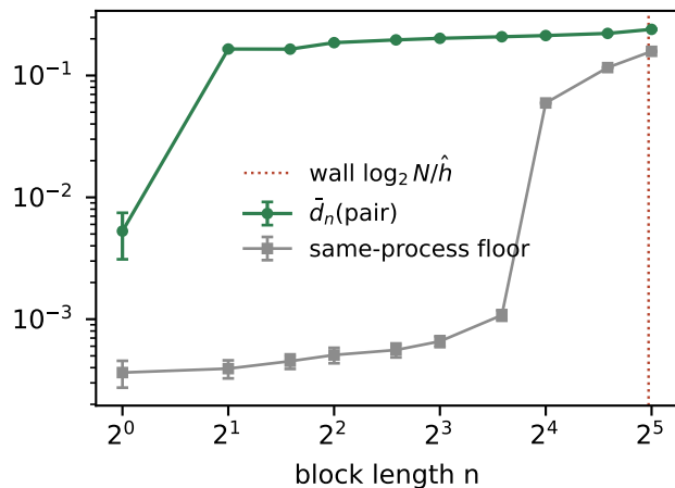
different task — emitted-token readout
