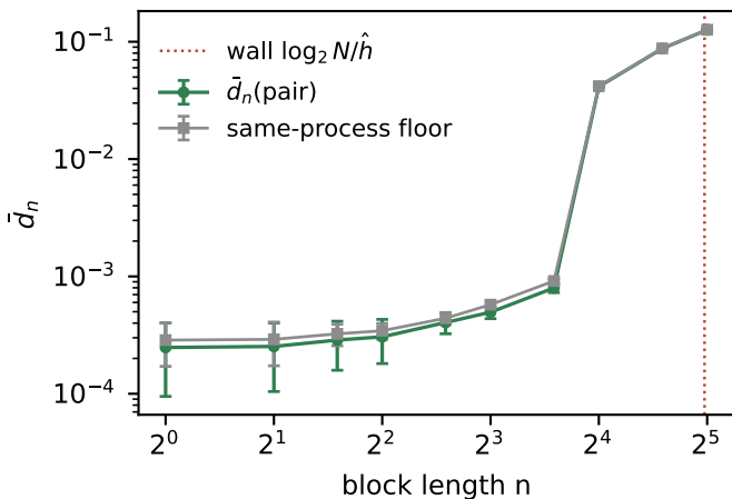
recoded null — emitted-token readout
