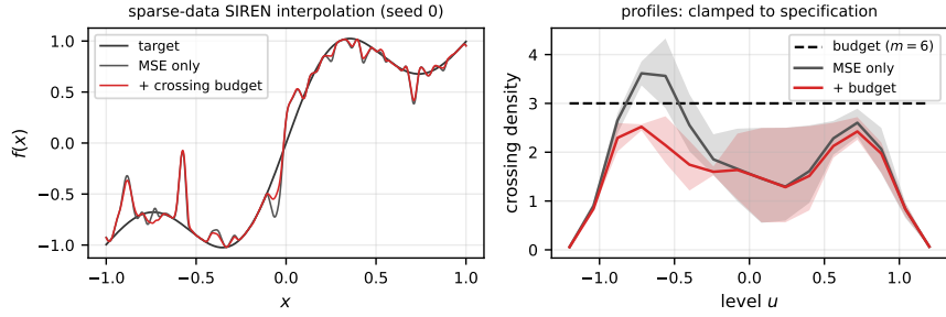
Figure 2: In-vitro positive control: sparse-data SIREN interpolation (left: seed-0 reconstructions; right: crossing profiles, min-max band over 3 seeds). MSE-only over-oscillates beyond budget; the one-sided budget clamps the profile within specification and improves test error on all seeds.
