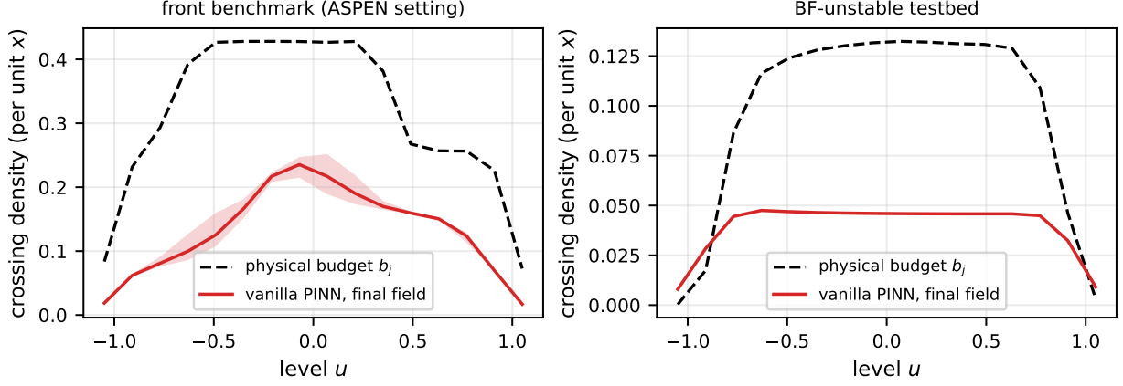
Figure 1: The diagnostic in action: measured crossing profiles versus physical budgets for the front benchmark (left; band = min-max over 3 seeds) and the BF-unstable testbed (right). Every failed vanilla field sits below budget—the under-oscillatory branch, on which one-sided budgets are by design inert.
