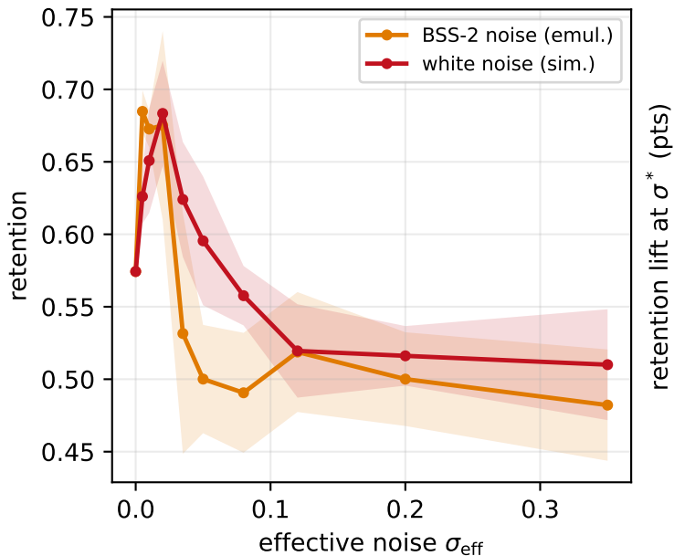
(a) inverted-U survives device-faithful BSS-2 noise (colored+6-bit+FP) — EMULATION
