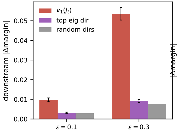
(a) directional interventions (M2)
