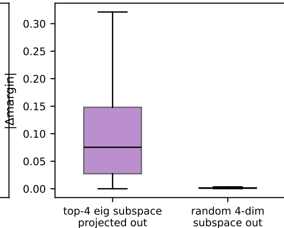
(b) slow-mode subspace ablation
