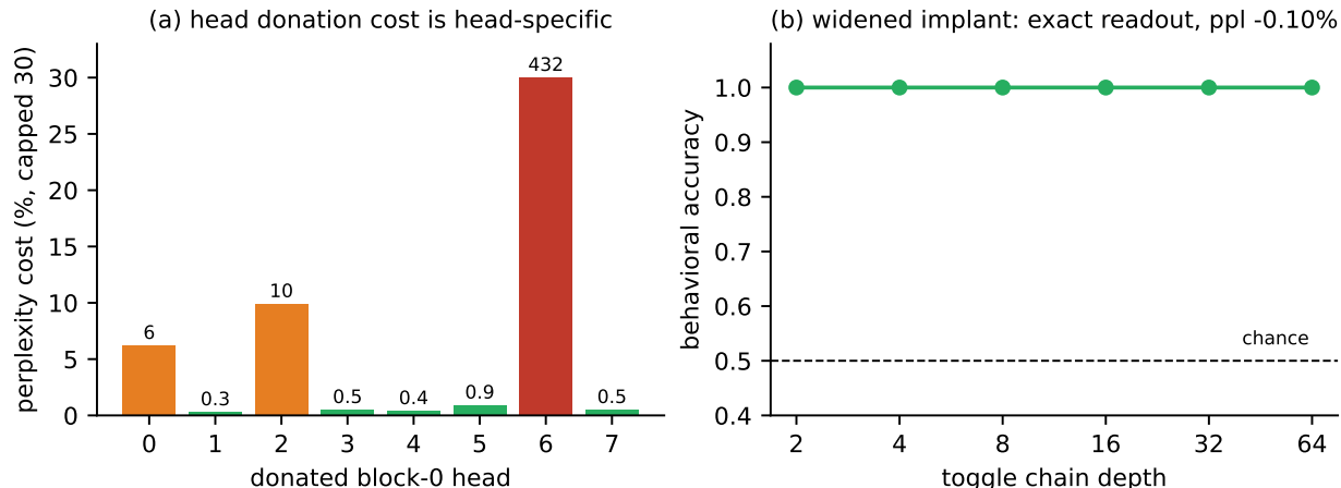
Figure 4: (a) Perplexity cost of donating each block-0 head (capped 30%; head 6 is 431.9%). (b) In the widened substrate the implanted circuit reads out at 1.00 through depth 64, at -0.098\% perplexity.
