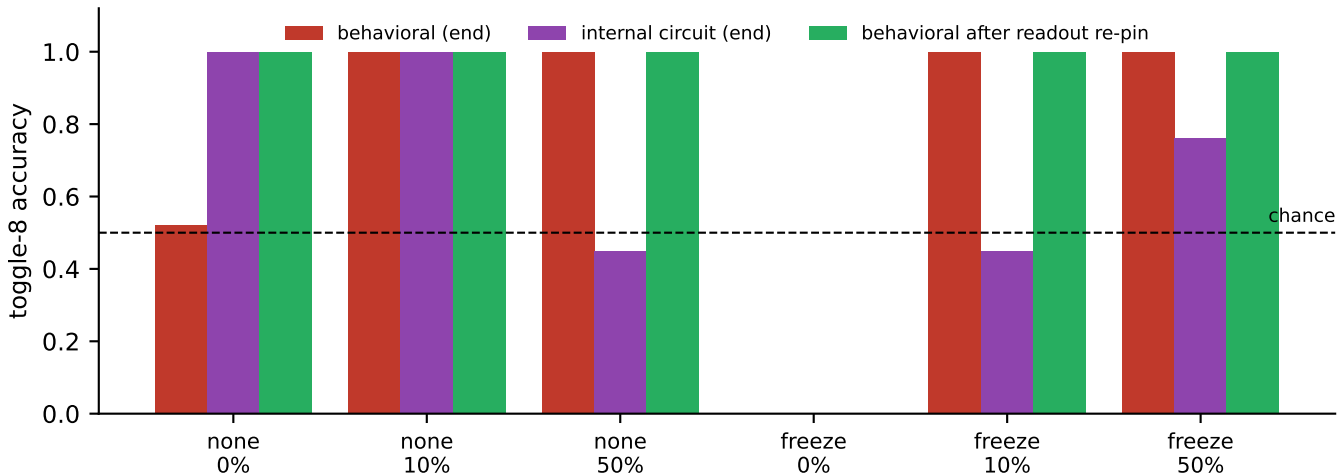
End-of-training state: concealed (recoverable) vs eroded vs protected
