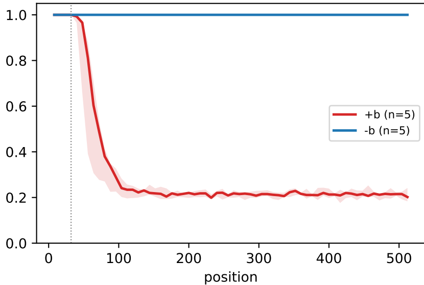
s5 ( n_h=4 )
