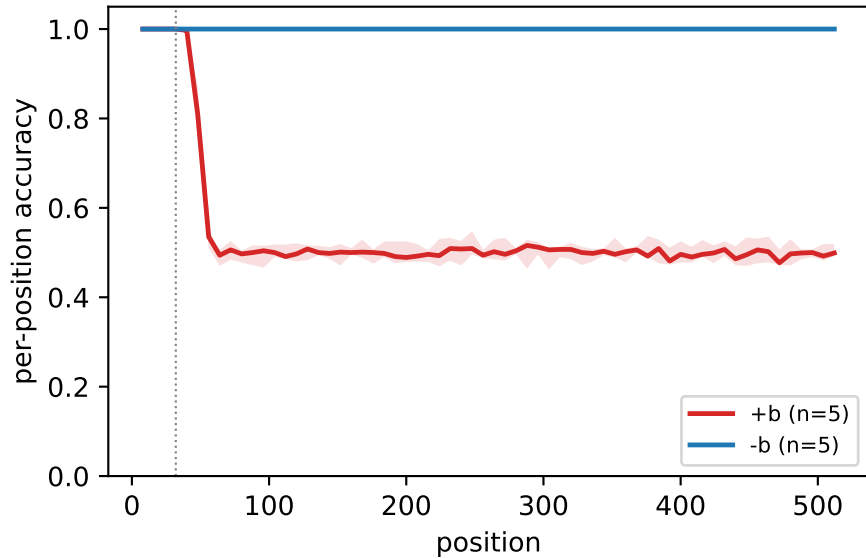
parity ( n_h=1 )
