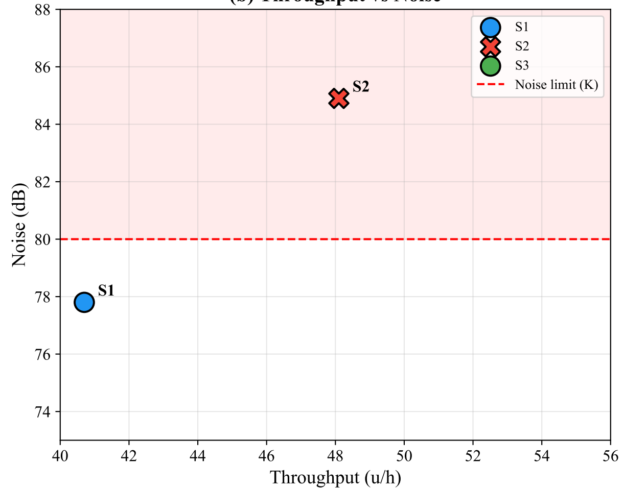
(b) Throughput vs Noise
