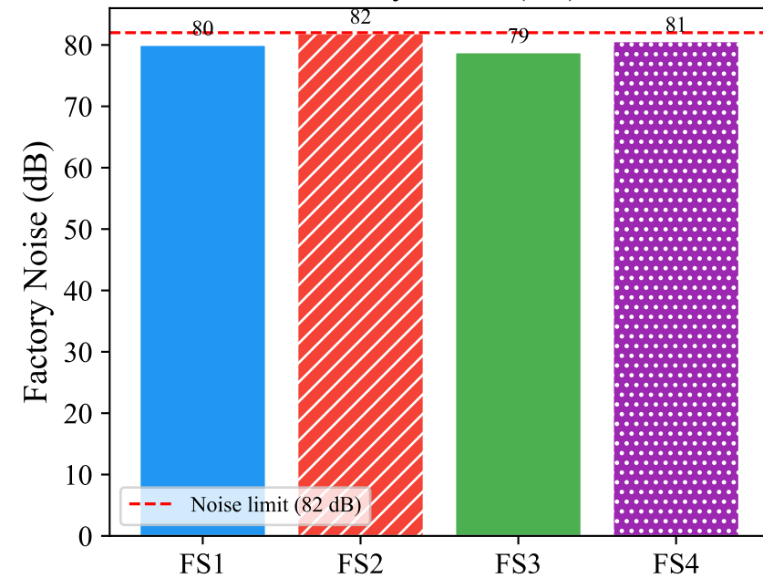
Factory Noise (dB)
