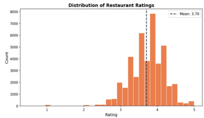
Fig 2: Rating Distribution
