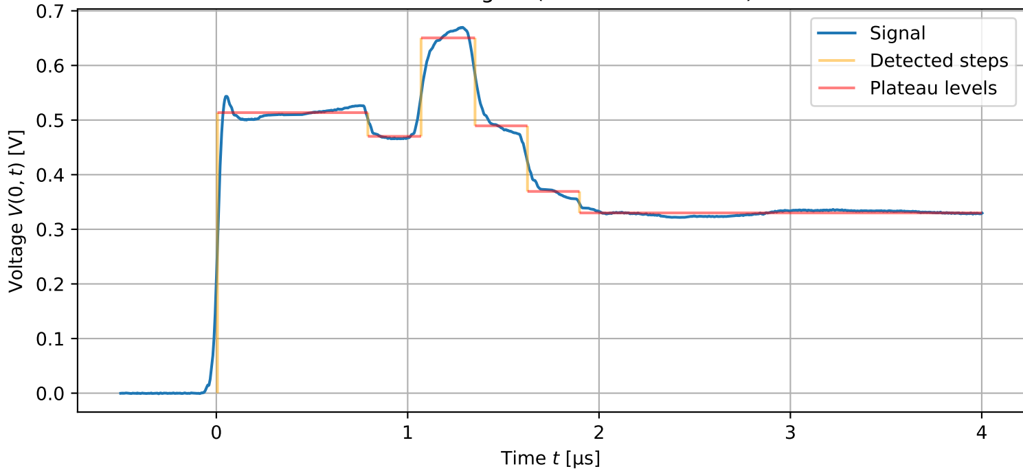
Measured signal (Circuit detective 1)
