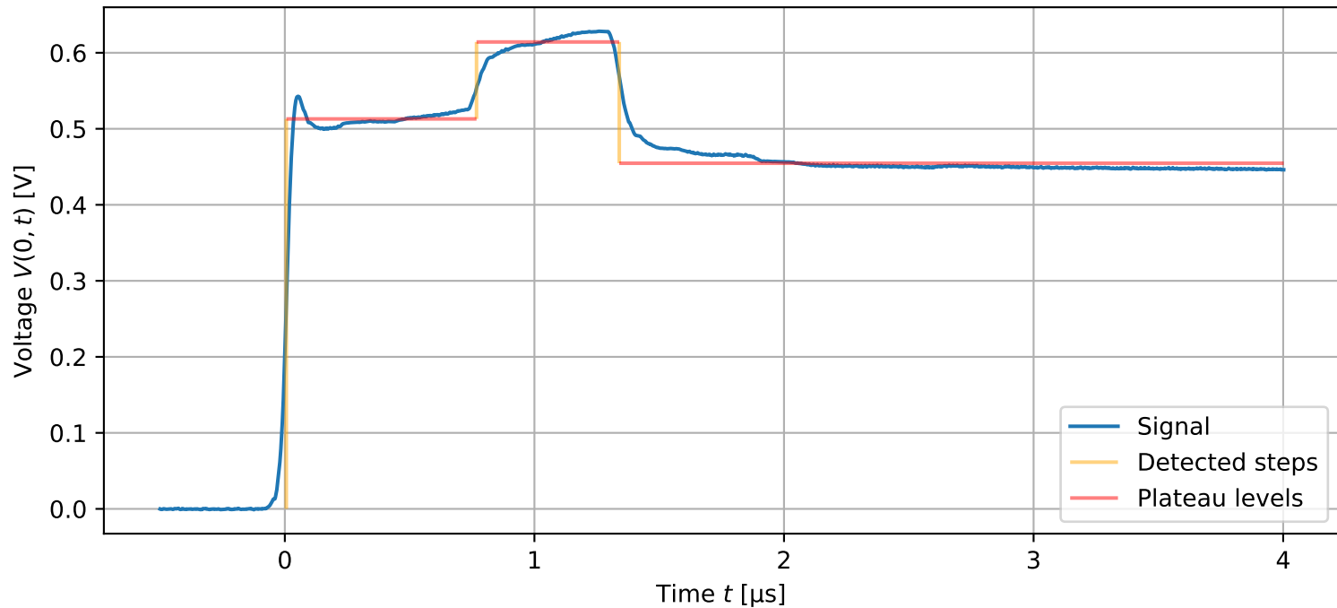
Measured signal (Circuit detective 2)
