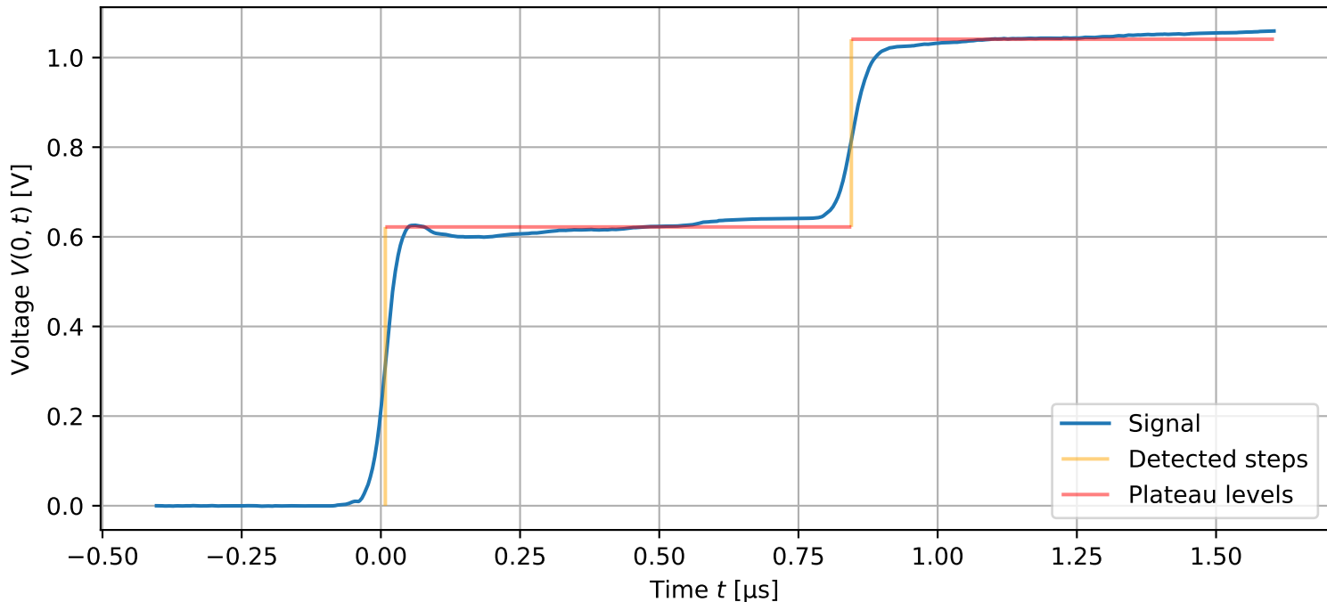
Measured signal (Cables 1 and 2 in series, open end)
