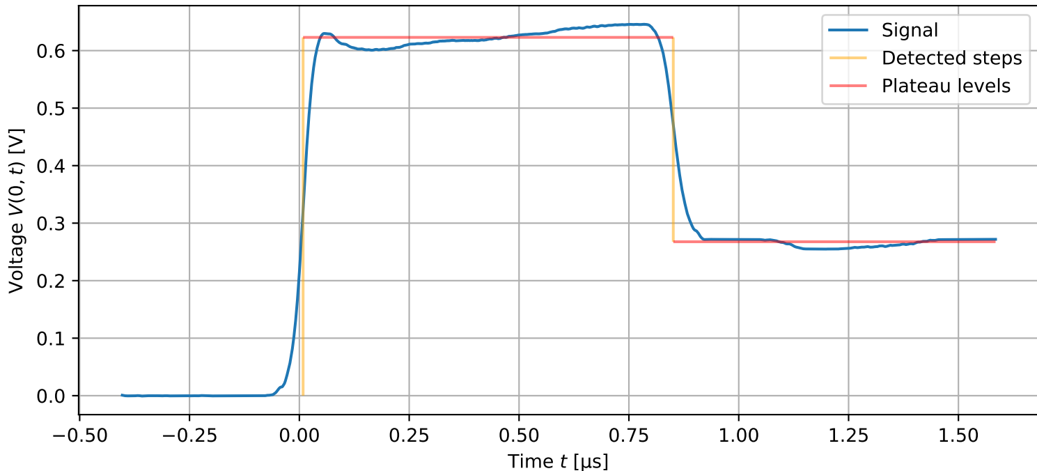
Measured signal (Cables 1 and 2 in series, short-circuited end)
