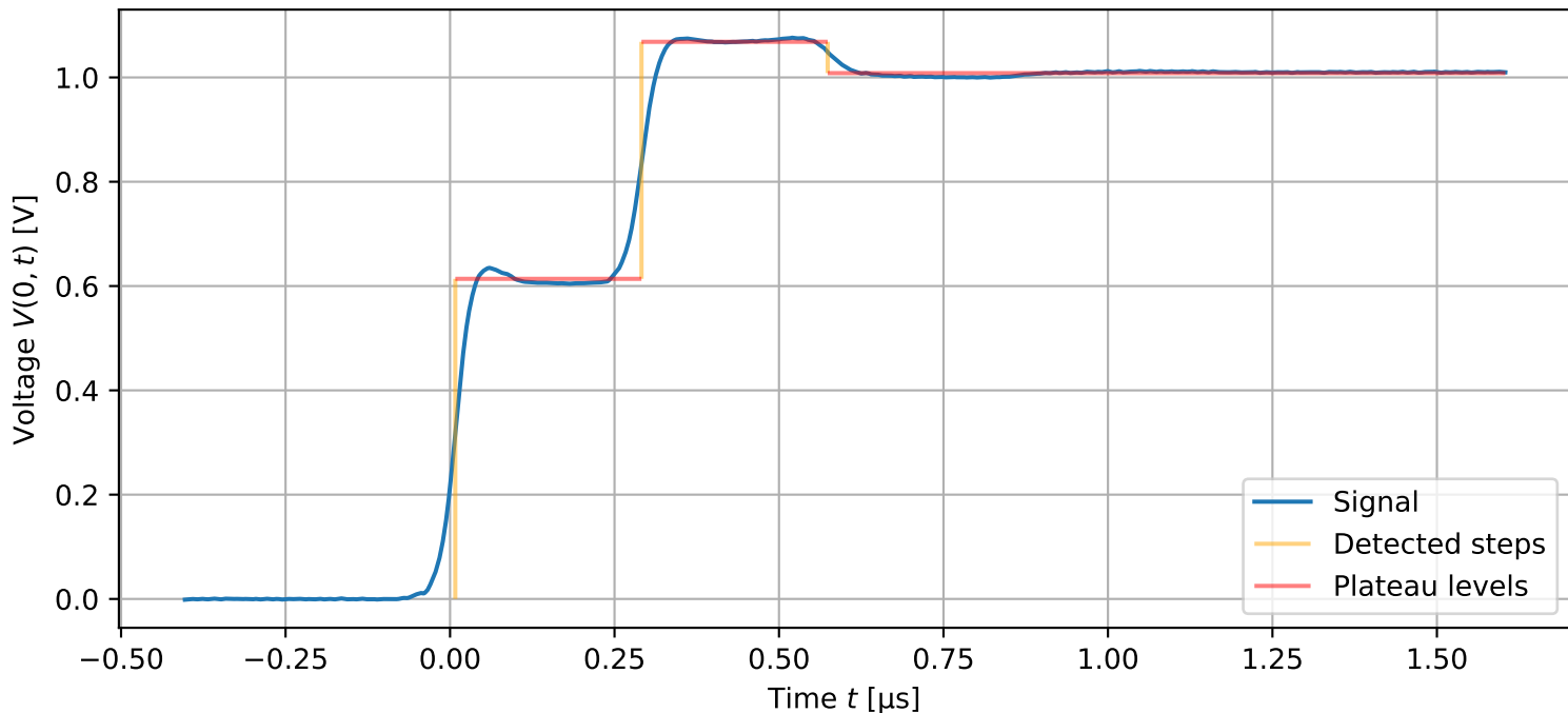
Measured signal (Cable 1, open end)
