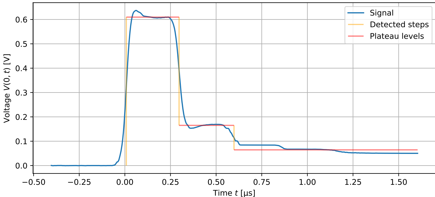
Measured signal (Cable 1, short-circuited end)
