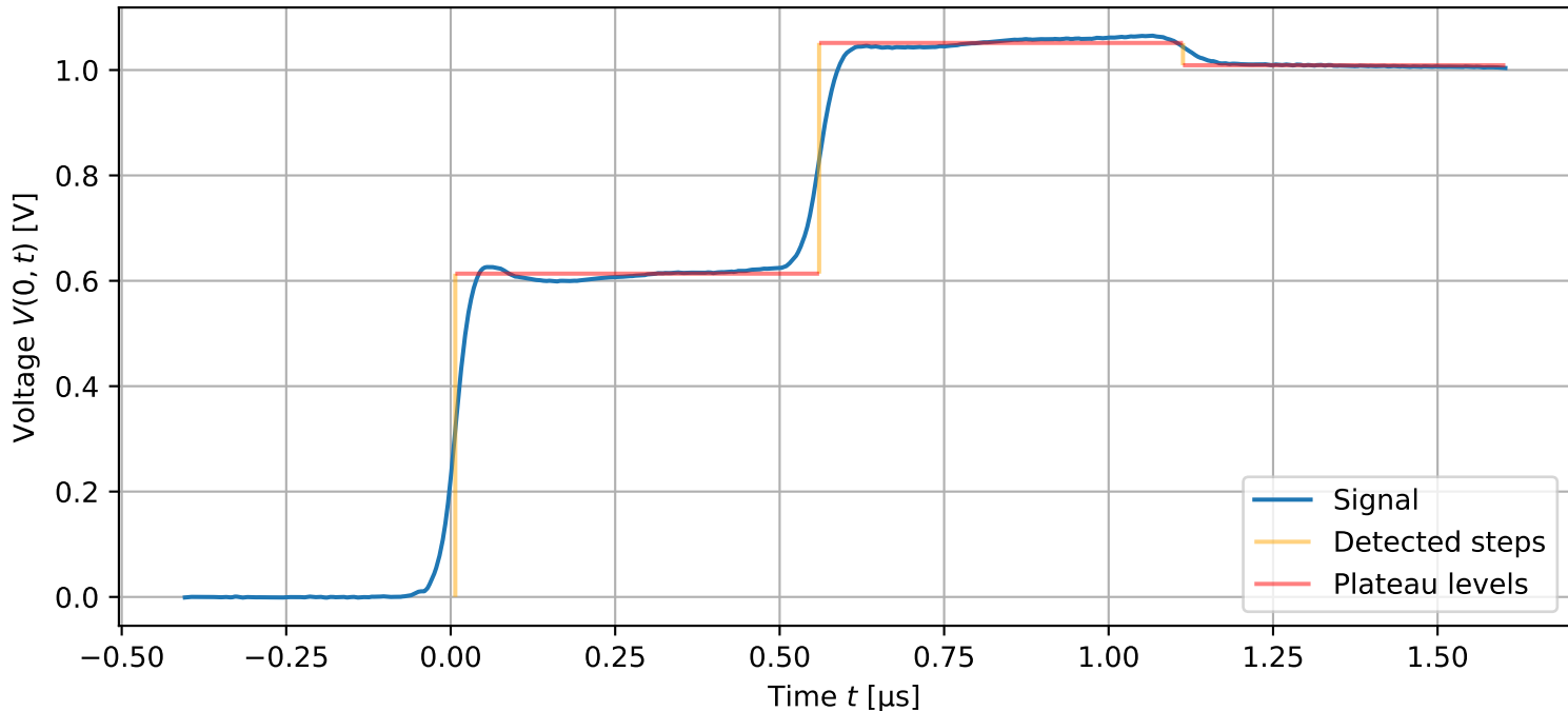
Measured signal (Cable 2, open end)
