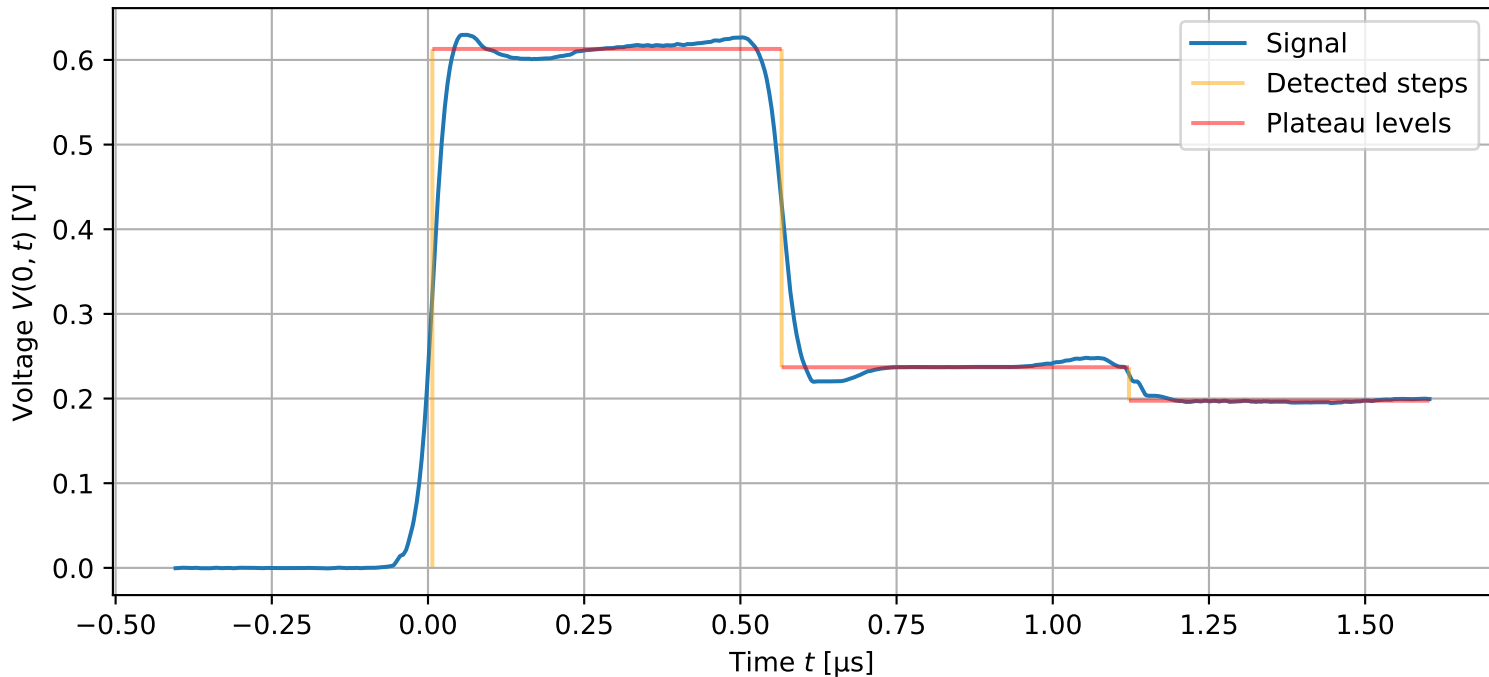
Measured signal (Cable 2, short-circuited end)
