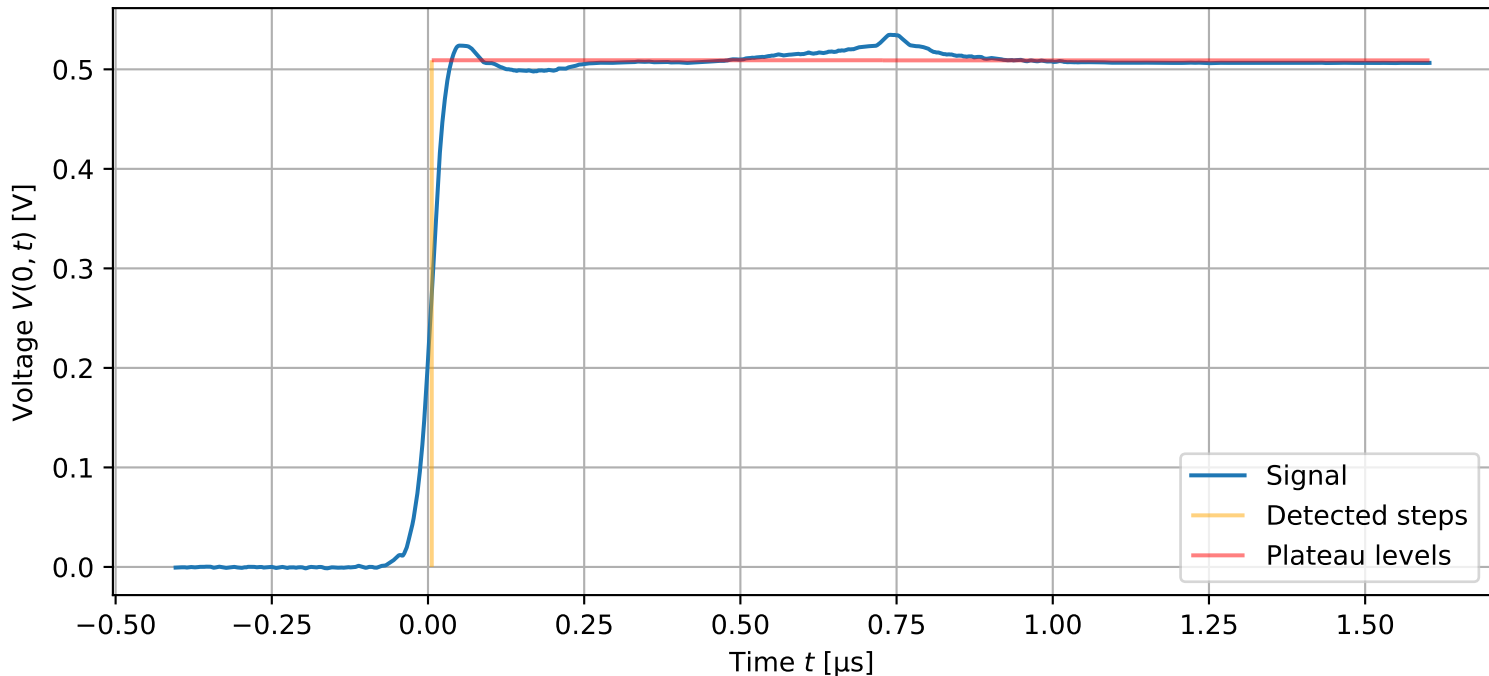
Measured signal (Cable 3, matched termination (50 \Omega ))
