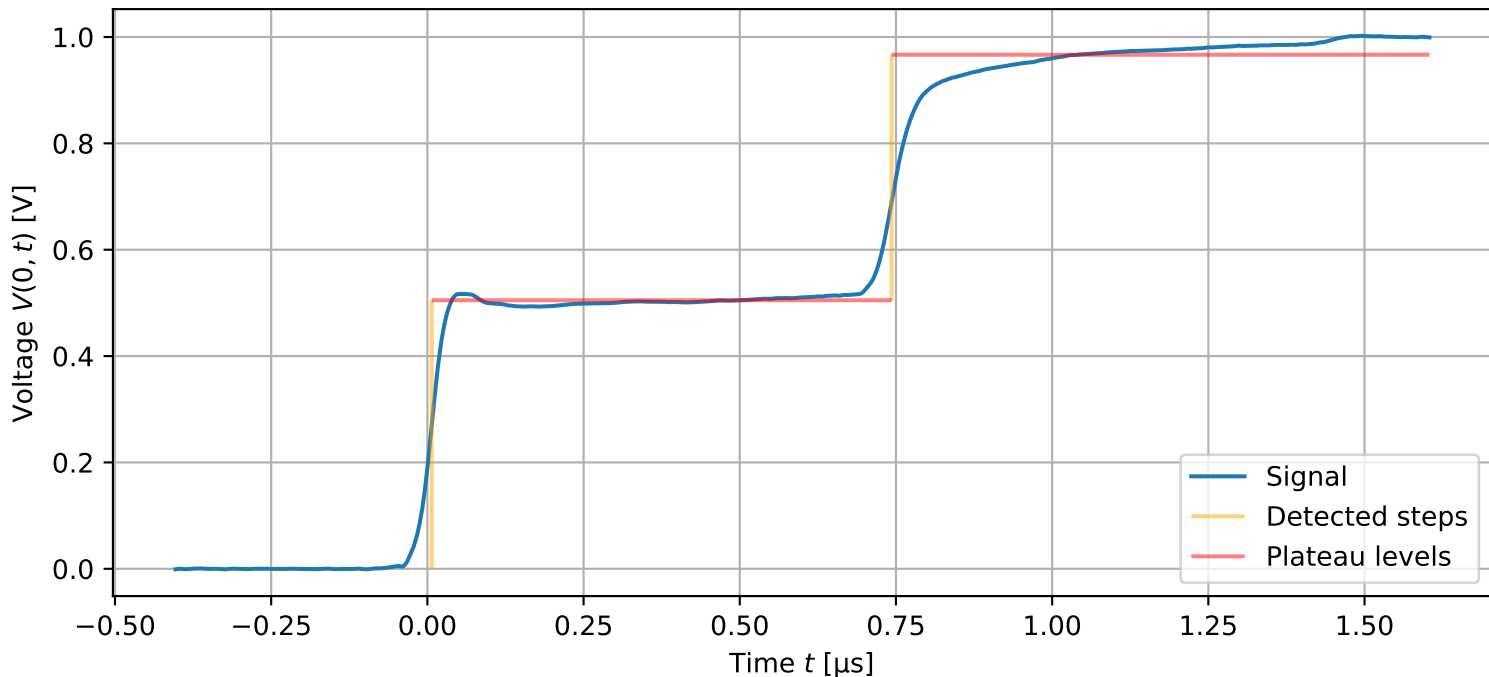
Measured signal (Cable 3, open end)
