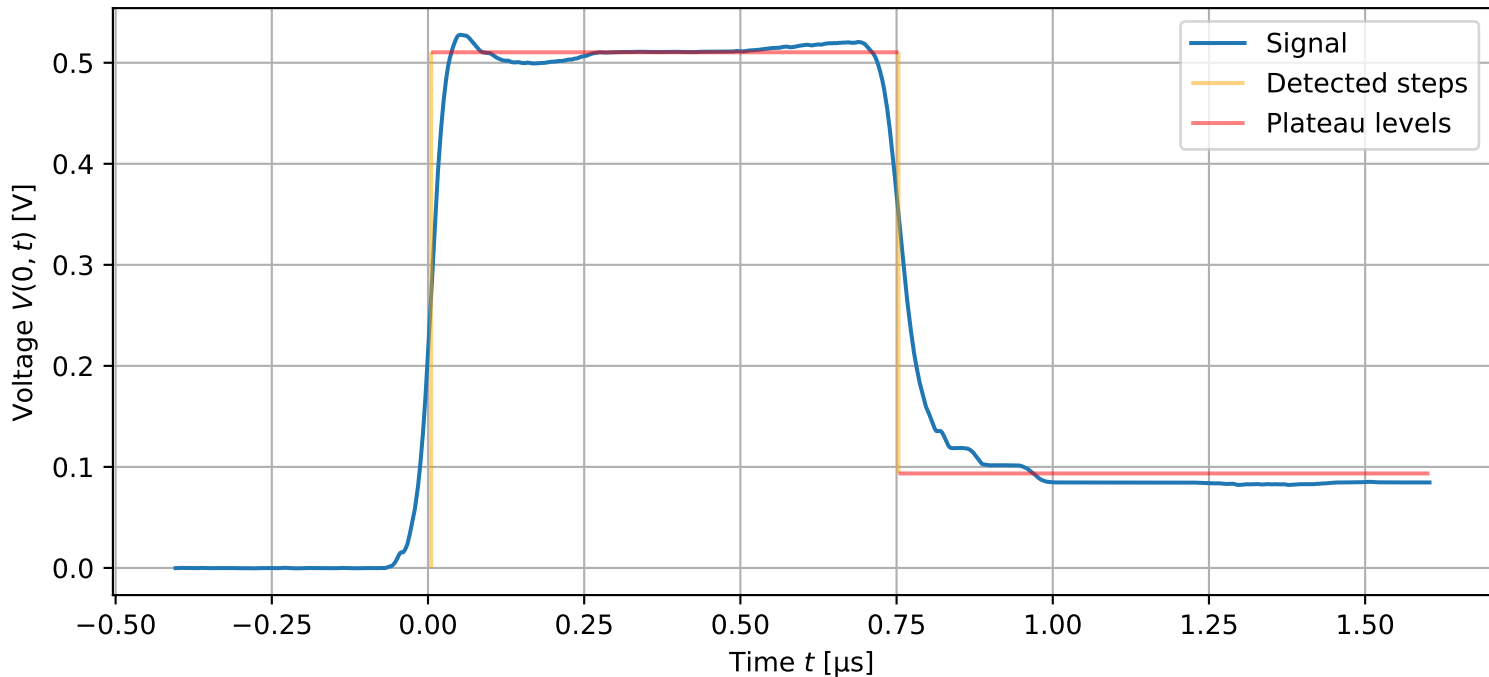
Measured signal (Cable 3, short-circuited end)
