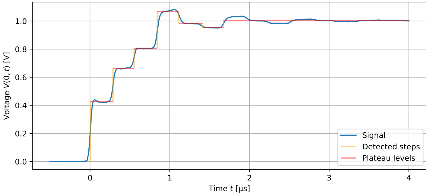
Measured signal (Splitter: both cables open)
