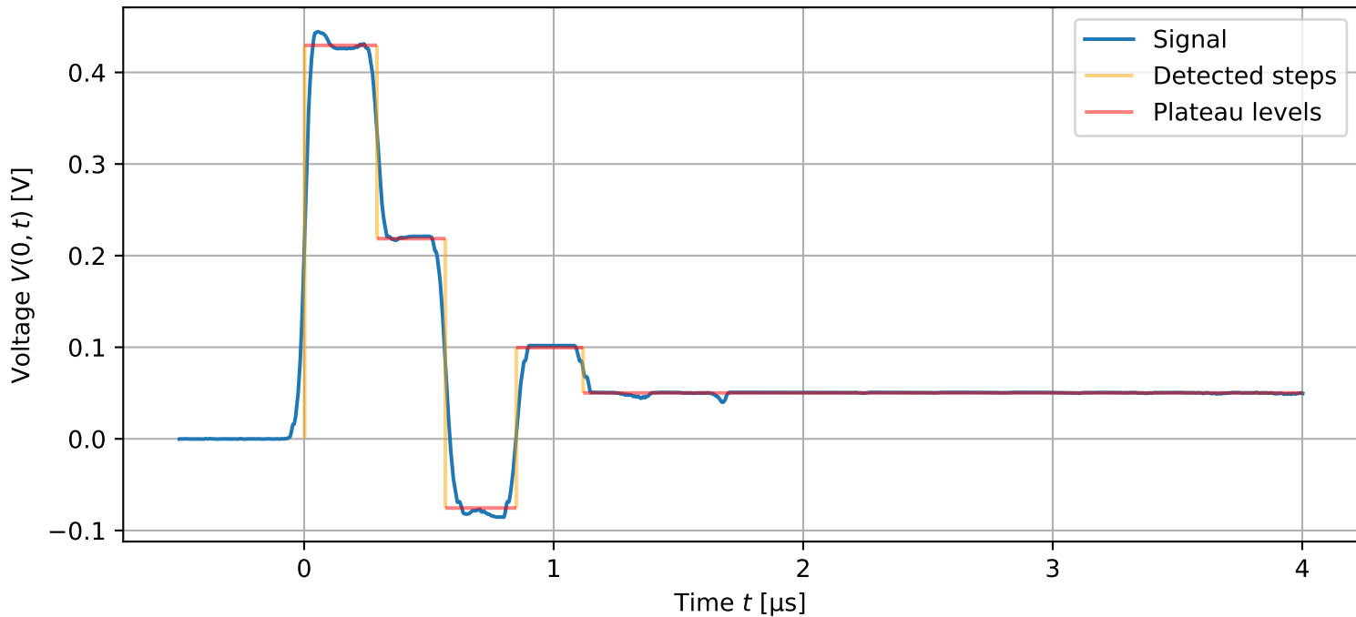
Measured signal (Splitter: both cables short-circuited)
