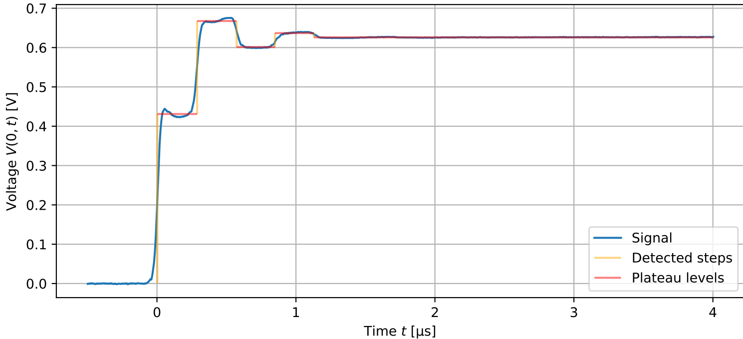
Measured signal (Splitter: cable 1 open, cable 2 matched)
