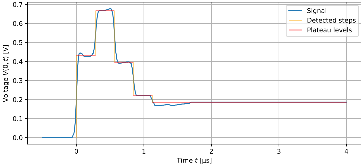
Measured signal (Splitter: cable 1 open, cable 2 short-circuited)
