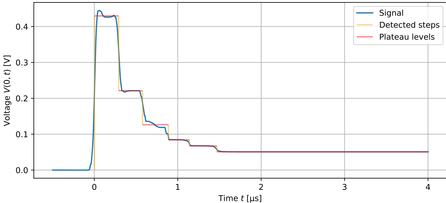
Measured signal (Splitter: cable 1 short-circuited, cable 2 matched)
