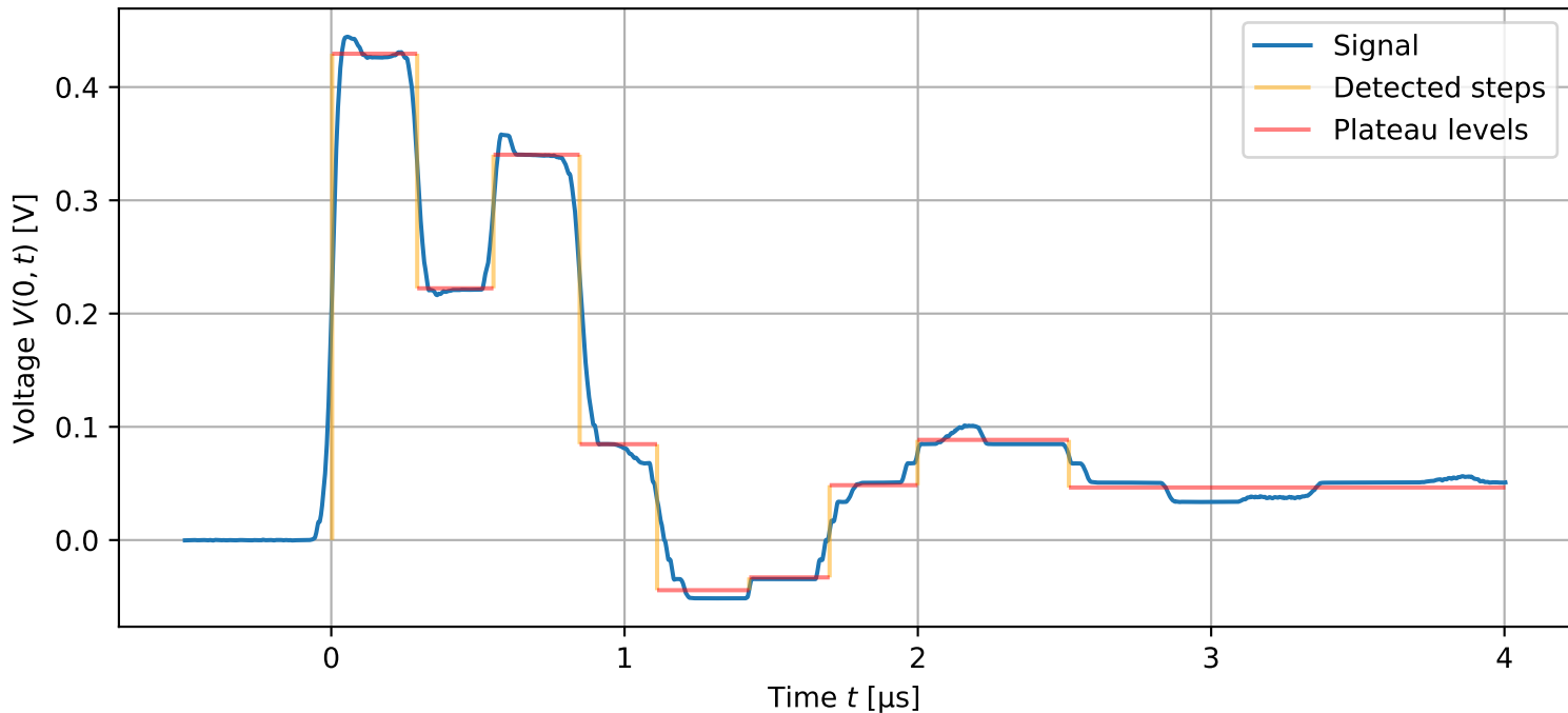
Measured signal (Splitter: cable 1 short-circuited, cable 2 open)
