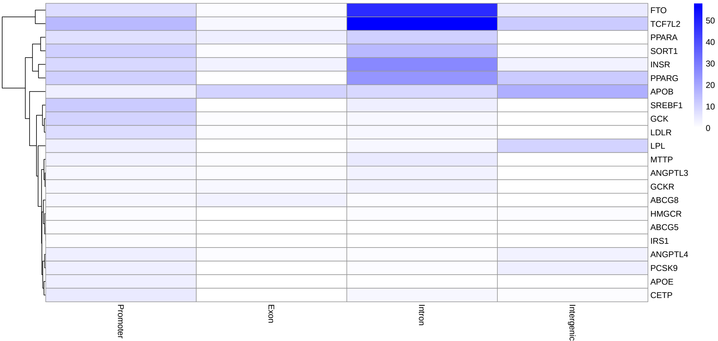
ATAC Peak Location per Cardiometabolic Gene
