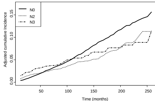
Supplementary Figure 18. Confounder-adjusted CIC of CIBC stratified by risk factors with violated PSH assumption in Black patients with IDC.
