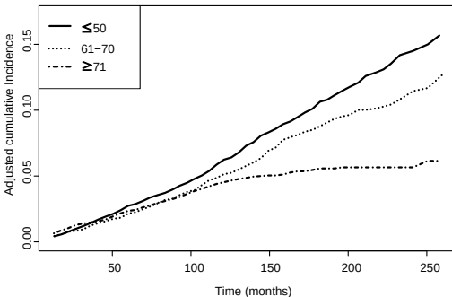
Supplementary Figure 18. Confounder-adjusted CIC of CIBC stratified by risk factors with violated PSH assumption in Black patients with IDC.
