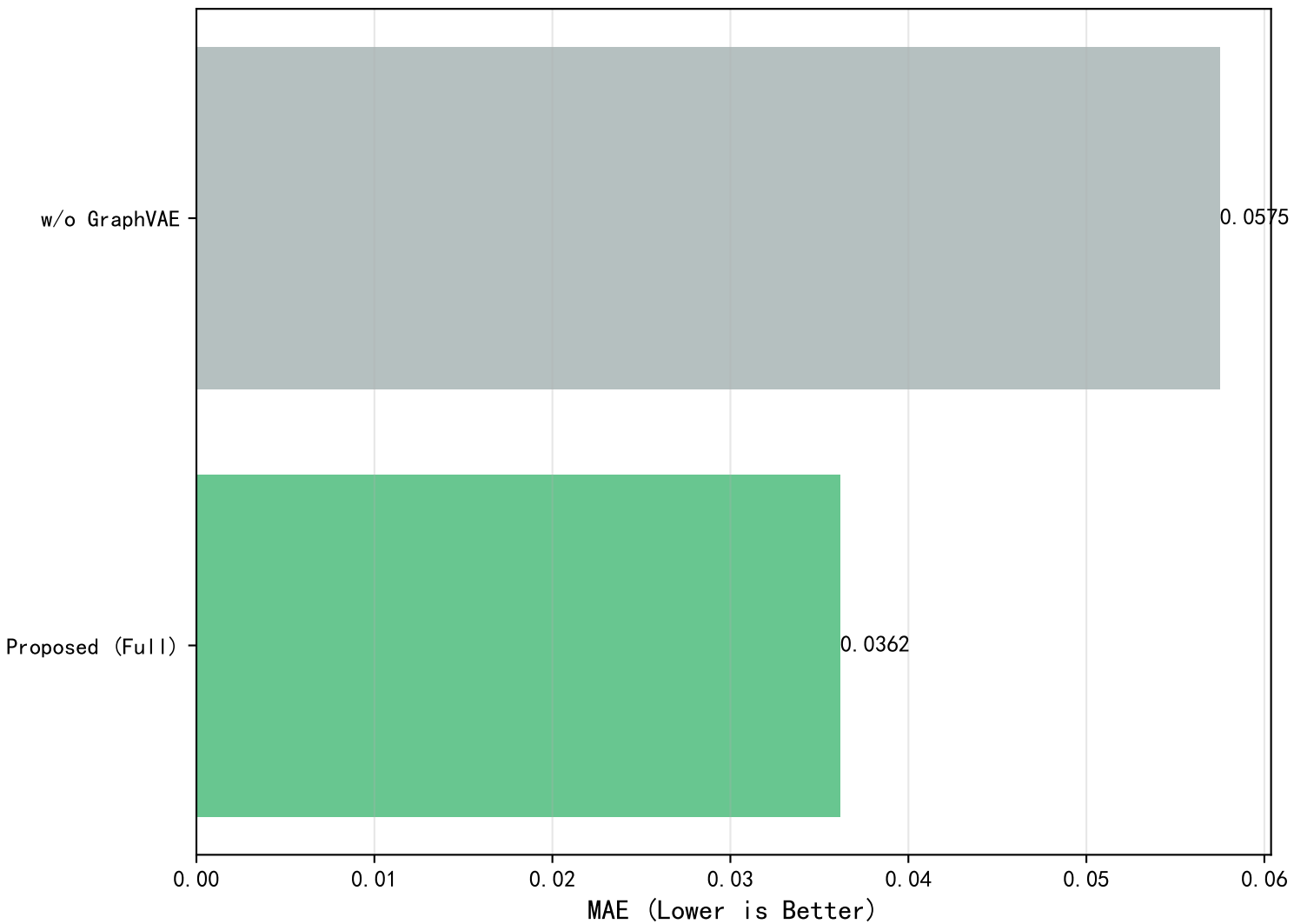
Ablation Study – Component Contribution
