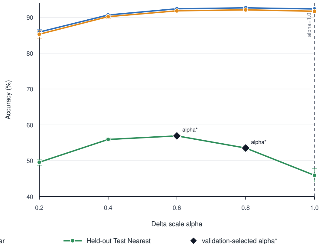
(b) ADI-DoRA
