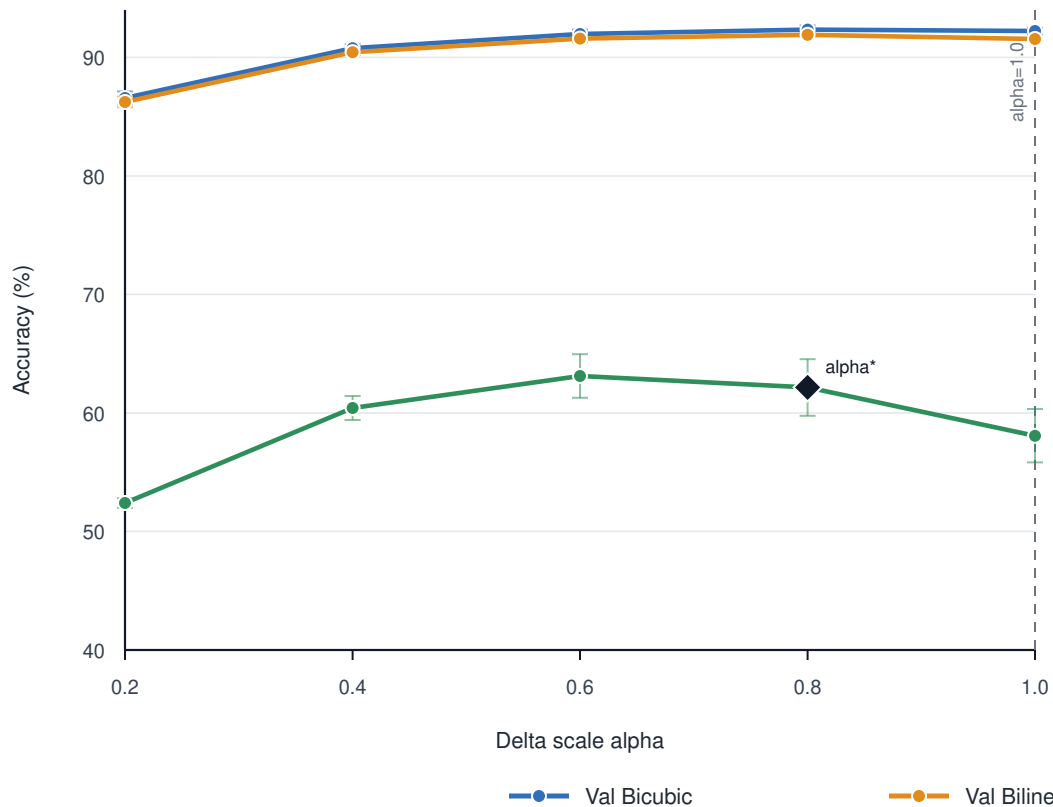
(a) ADI-LoRA
