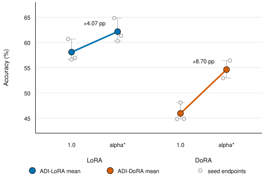
Held-out Nearest accuracy
