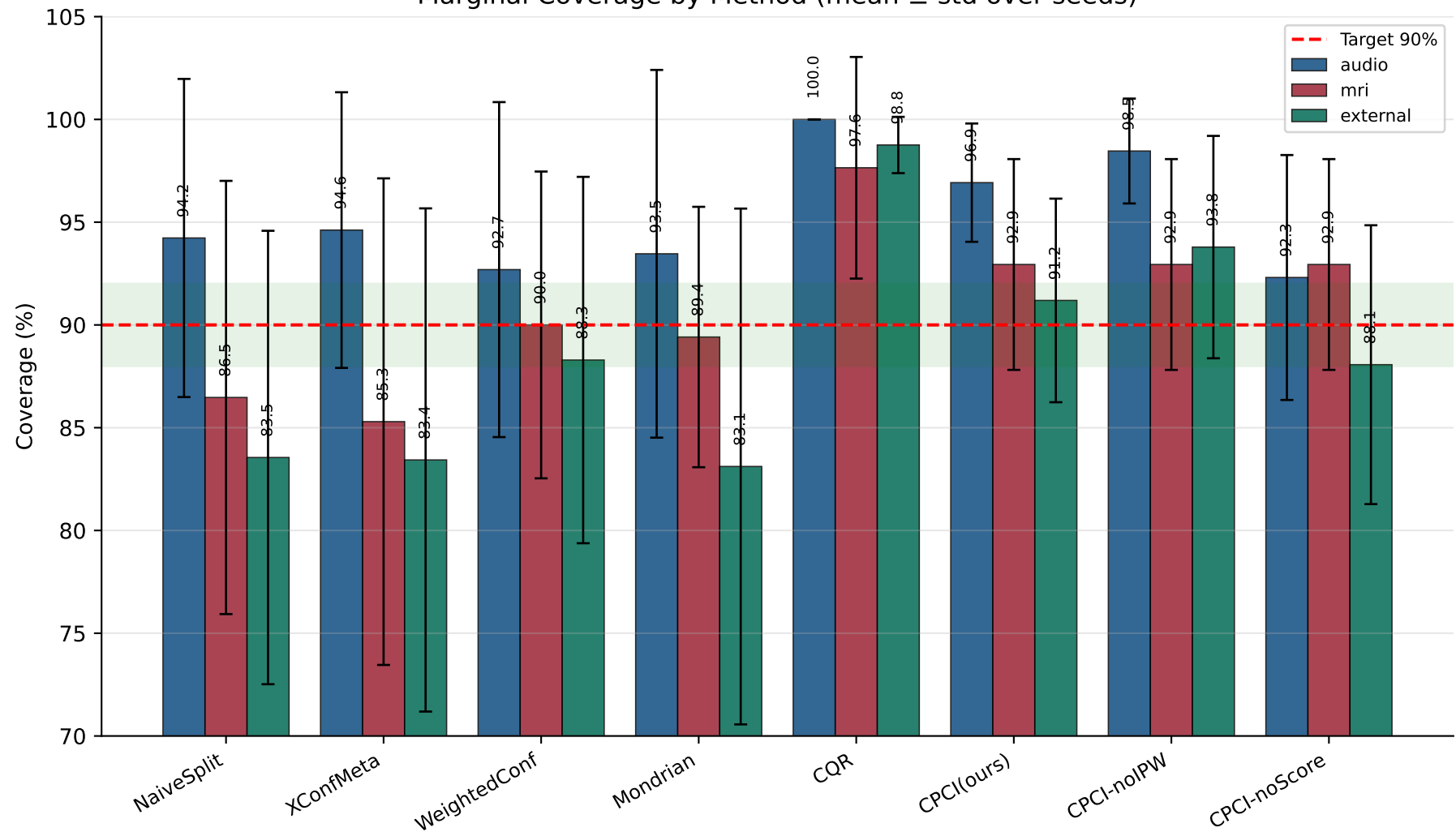
Marginal Coverage by Method (mean \pm std over seeds)
