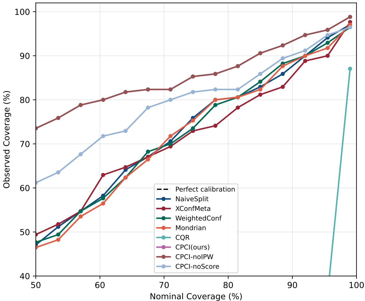
Calibration Curve (mri, pooled over seeds) intervals built from calibration scores only
