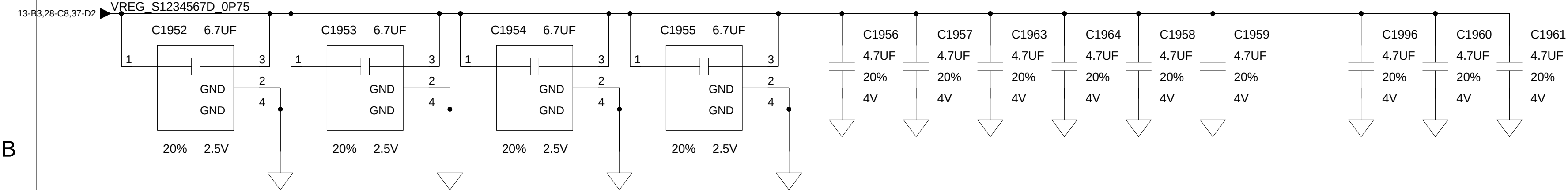
APC2 - PWR Dedicated sense pins on package
