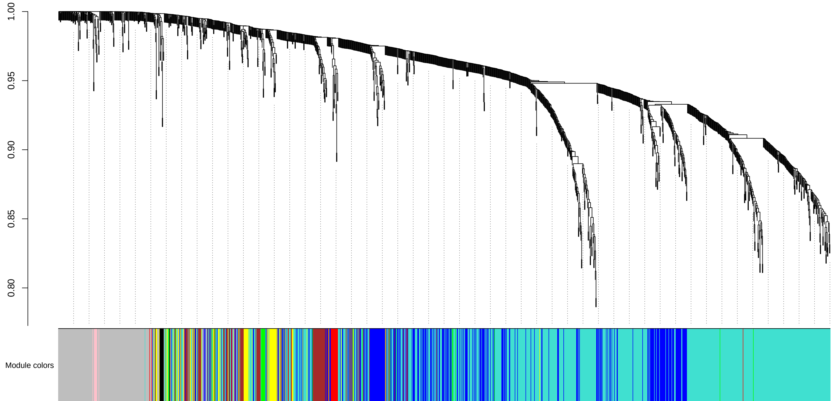
Gene dendrogram and module colors (Signed Network)
