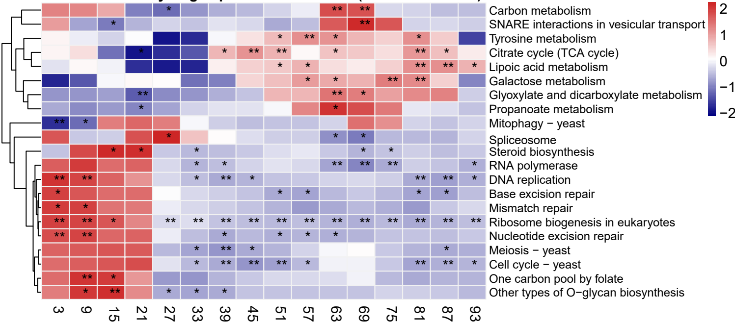
Hydrogen peroxide vs Control (GAM Cumulative)
