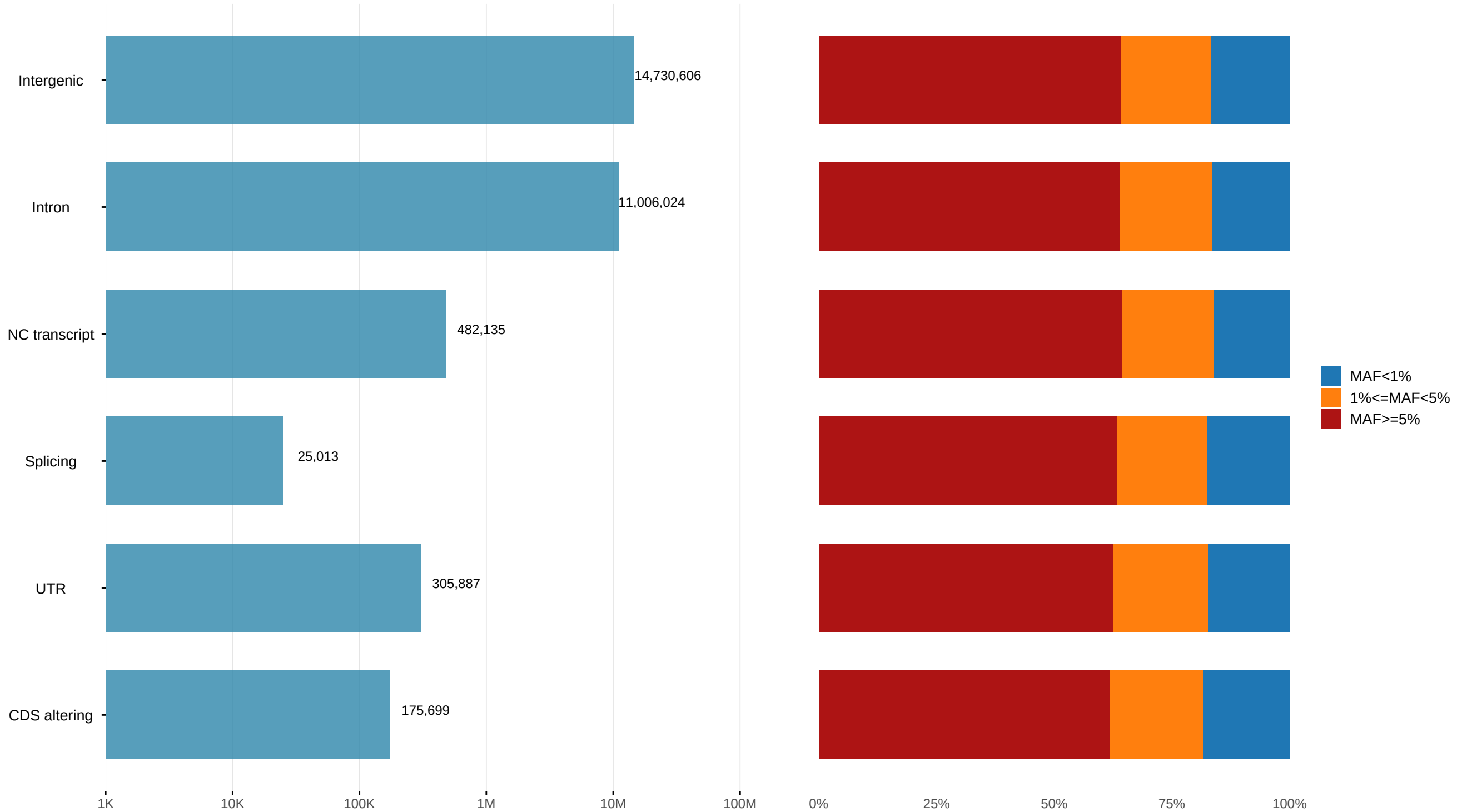
SNPs Distribution with Gene locus and MAF
