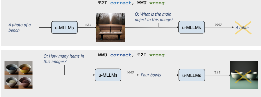
Figure 1: The imbalance between Text-to-Image Generation (T2I) and Multi-modal Understanding (MMU). For the same image, unified multimodal models may struggle to perform both generation and understanding consistently.
