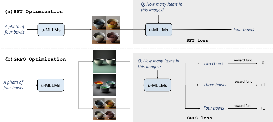
Figure 2: Training pipeline of UniRL (a) SFT Optimization: A prompt is used to generate a single image, which, together with the corresponding question, is used to predict an answer and compute the SFT loss. (b) GRPO Optimization: The same prompt generates a set of images, each paired with the same question to produce multiple answers, which are used to compute the GRPO loss.
