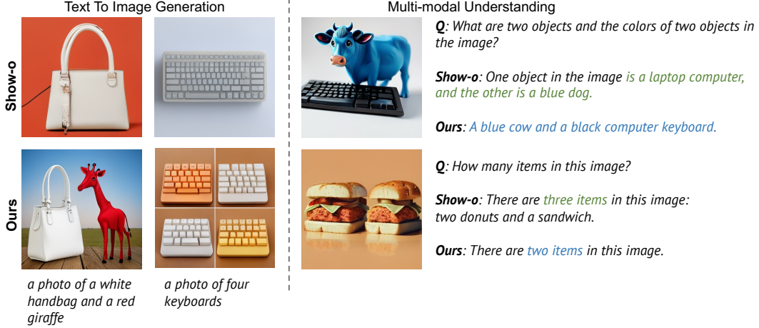
Figure 3: Qualitative comparison of our method with the original models on both text-to-image generation (T2I) and multimodal understanding (MMU) tasks.
