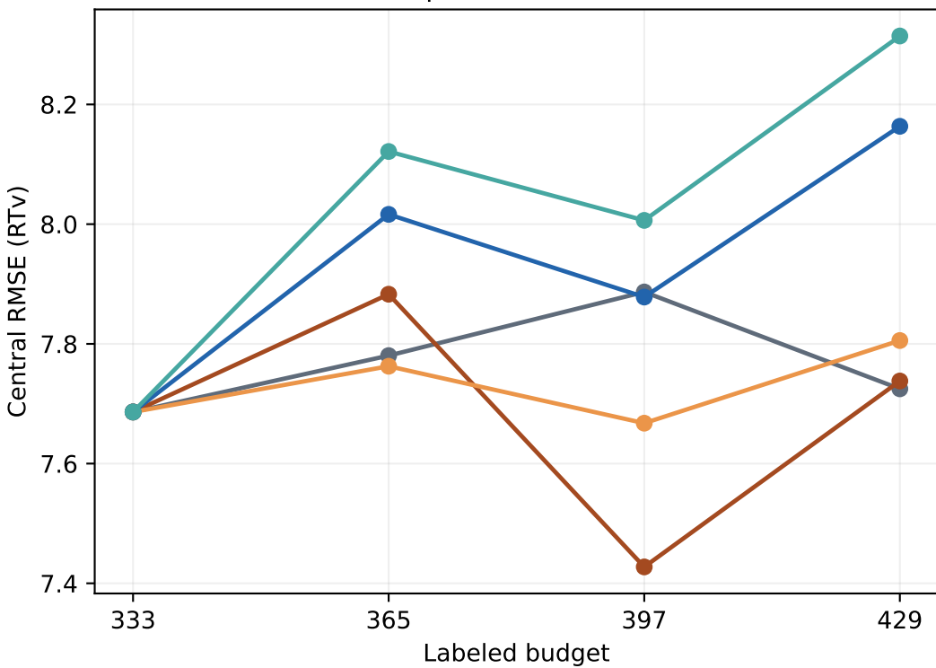
Validation | initialization seed 525
