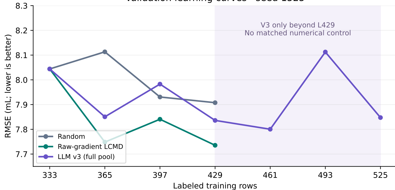
Validation learning curves · seed 1525
